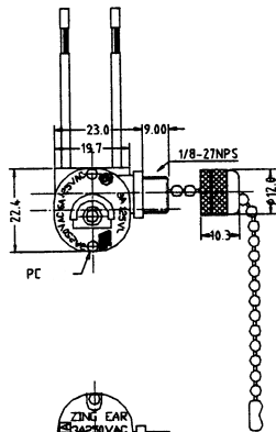
Mounting Hole: 0.406"
